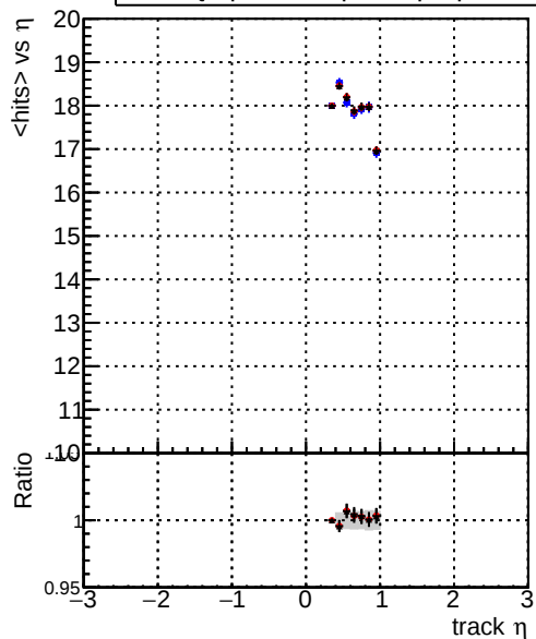
mean hit — DQM_original_step2_pt1000_eta0p4to1p0 — DQM_mkFit_step2_pt1000_eta0p4to1p0 — DQM_pixelCPETemplate_step2_pt1000_eta0p4to1p0
