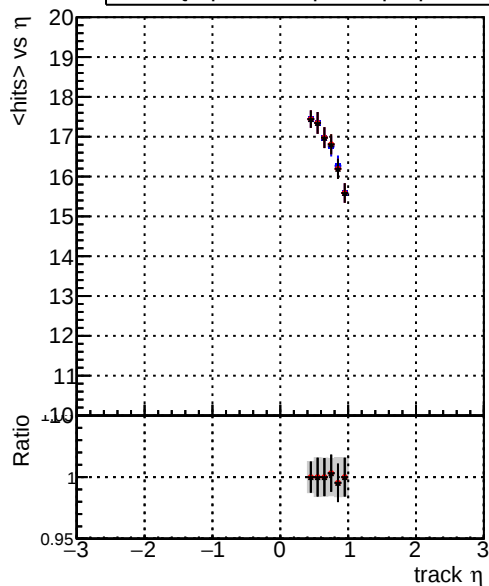
mean hit — DQM_original_step2_pt1000_eta0p4to1p0 — DQM_mkFit_step2_pt1000_eta0p4to1p0 — DQM_pixelCPETemplate_step2_pt1000_eta0p4to1p0
