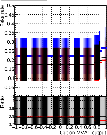
Fake rate vs. MVA1
