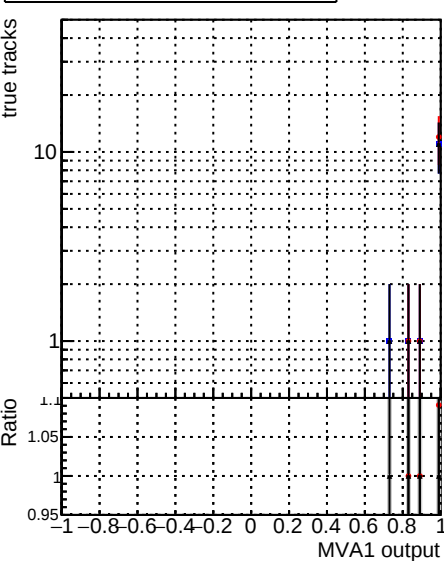
N of associated tracks (recoToSim) vs MVA1
