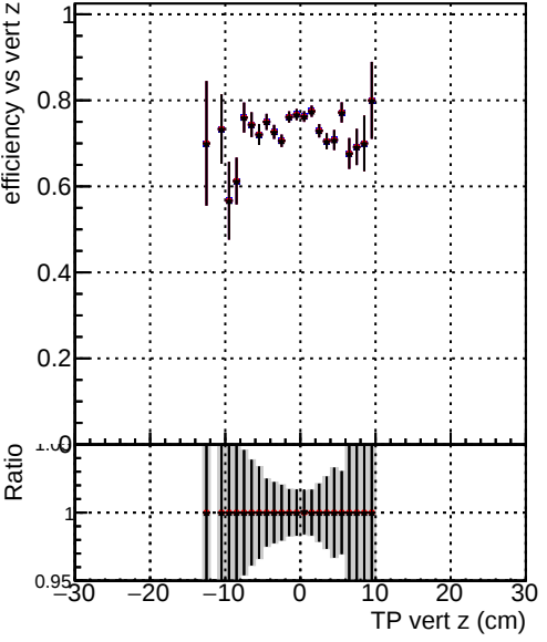
Efficiency vs vert z Legend: DQM_original_step2_pt1000_eta0p4to1p0 DQM_mkFit_step2_pt1000_eta0p4to1p0 DQM_pixelCPETemplate_step2_pt1000_eta0p4to1p0
