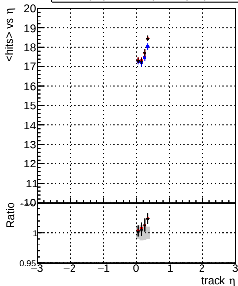
mean hit — DQM_original_step2_pt1000_eta0p0to0p4 — DQM_mkFit_step2_pt1000_eta0p0to0p4 — DQM_pixelCPEtemplate_step2_pt1000_eta0p0to0p4
