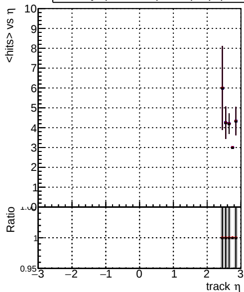
mean hits vs \eta DQM_original_step2_pt0p1to1_eta2p5to4p0 DQM_mkFit_step2_pt0p1to1_eta2p5to4p0 DQM_pixelCPEtemplate_step2_pt0p1to1_eta2p5to4p0
