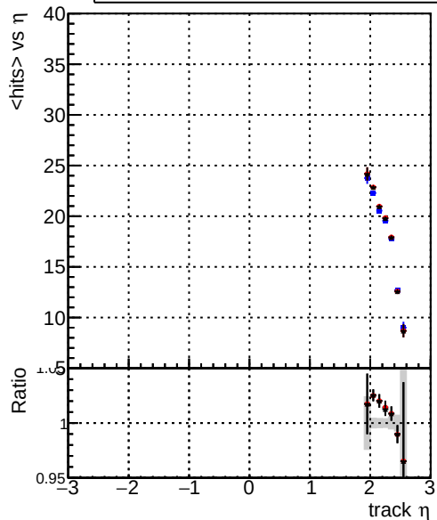
mean hits — DQM_original_step2_pt0p1to1_eta2p0to2p5 — DQM_mkFit_step2_pt0p1to1_eta2p0to2p5 — DQM_pixelCPETemplate_step2_pt0p1to1_eta2p0to2p5
