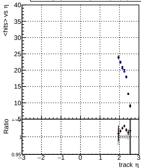
mean hit — DQM_original_step2_pt0p1to1_eta2p0to2p5 — DQM_mkFit_step2_pt0p1to1_eta2p0to2p5 — DQM_pixelCPETemplate_step2_pt0p1to1_eta2p0to2p5
