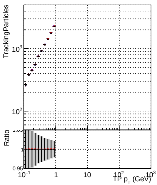
—•— DQM_original_step2_pt0p1to1_eta2p0to2p5 —•— DQM_mkFit_step2_pt0p1to1_eta2p0to2p5 —•— DQM_pixelCPETemplate_step2_pt0p1to1_eta2p0to2p5
