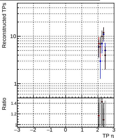
—•— DQM_original_step2_pt0p1to1_eta2p0to2p5 —•— DQM_mkFit_step2_pt0p1to1_eta2p0to2p5 —•— DQM_pixelCPETemplate_step2_pt0p1to1_eta2p0to2p5
