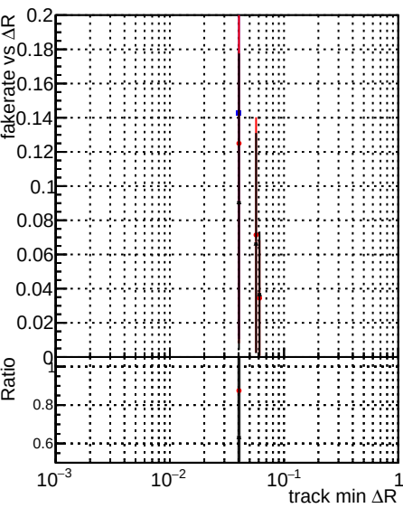
Fake rate vs \Delta R(\text{track}, \text{jet}) DQM_original step2_pt0p1to1_eta2p0to2p5 DQM_mkFit step2_pt0p1to1_eta2p0to2p5 DQM_pixelCPETemplate step2_pt0p1to1_eta2p0to2p5
