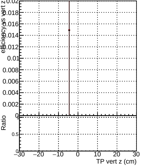
Efficiency vs TP vert z Legend: DQM_original_step2_pt0p1to1_eta2p0to2p5 DQM_mkFit_step2_pt0p1to1_eta2p0to2p5 DQM_pixelCPETemplate_step2_pt0p1to1_eta2p0to2p5
