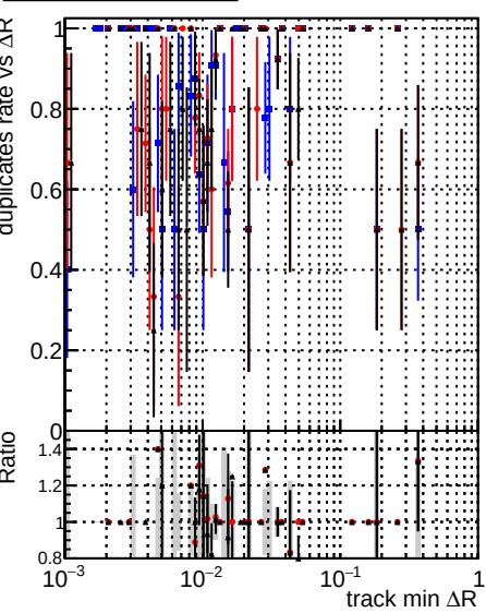
Legend: DQM original step2 pt0p1to1 eta1p6to2p0 (blue), DQM mkFit step2 pt0p1to1 eta1p6to2p0 (red), DQM pixelCPETemplate step2 pt0p1to1 eta1p6to2p0 (black)
