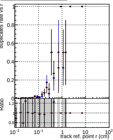
—•— DQM_original_step2_pt0p1to1_eta1p6to2p0 —•— DQM_mkFit_step2_pt0p1to1_eta1p6to2p0 —•— DQM_pixelCPETemplate_step2_pt0p1to1_eta1p6to2p0
