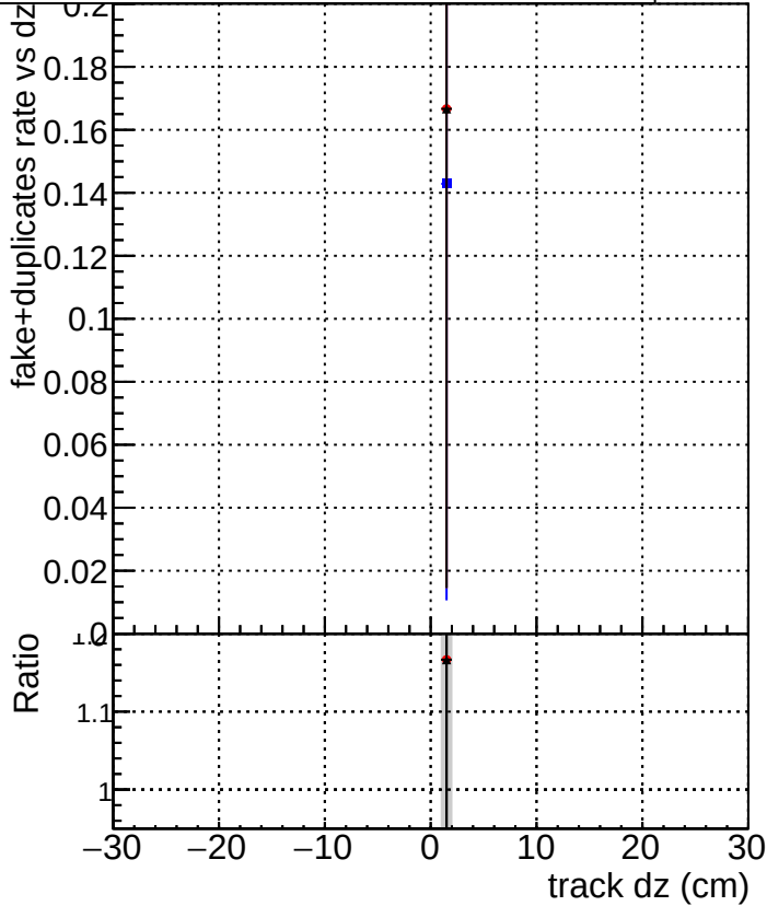
DQM_original_step2_pt0p1to1_eta1p6to2p0 DQM_mkFit_step2_pt0p1to1_eta1p6to2p0 DQM_pixelCPETemplate_step2_pt0p1to1_eta1p6to2p0
