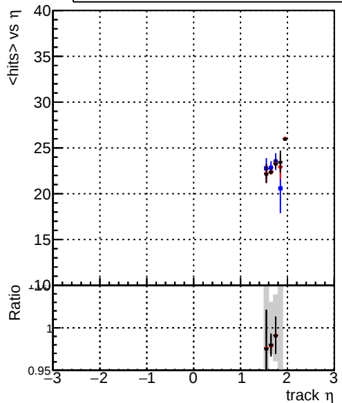
— DQM_original_step2_pt0p1to1_eta1p6to2p0 — DQM_mkFit_step2_pt0p1to1_eta1p6to2p0 — DQM_pixelCPETemplate_step2_pt0p1to1_eta1p6to2p0 mean hits
