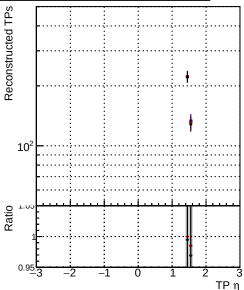
● DQM_original_step2_pt0p1to1_eta1p4to1p6 ● DQM_mkFit_step2_pt0p1to1_eta1p4to1p6 ● DQM_pixelCPETemplate_step2_pt0p1to1_eta1p4to1p6
