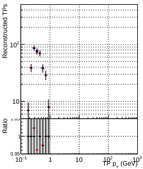
● DQM_original_step2_pt0p1to1_eta1p4to1p6 ● DQM_mkFit_step2_pt0p1to1_eta1p4to1p6 ● DQM_pixelCPETemplate_step2_pt0p1to1_eta1p4to1p6
