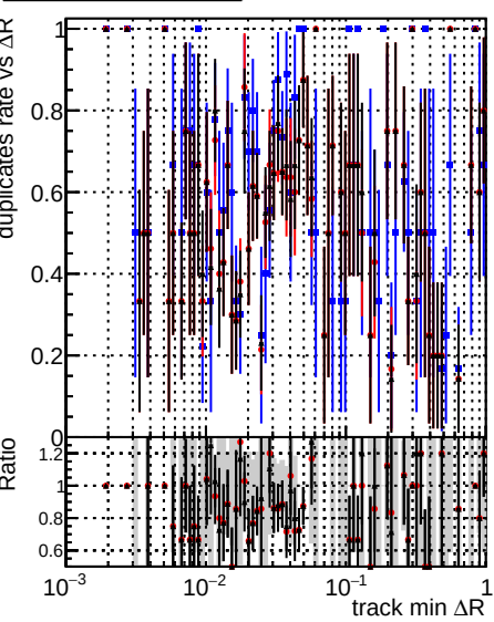
Legend: DQM original step2_pt0p1to1_eta1p4to1p6 (blue), DQM mkFit step2_pt0p1to1_eta1p4to1p6 (red), DQM pixelCPE template step2_pt0p1to1_eta1p4to1p6 (black)
