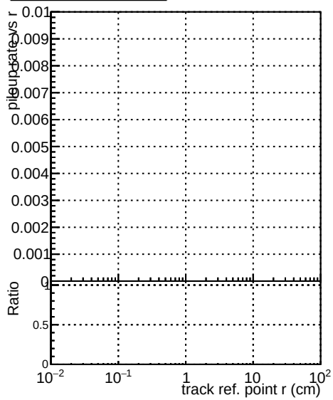
Legend: - DQM_original_step2_pt0p1to1_eta1p4to1p6 - DQM_mkFit_step2_pt0p1to1_eta1p4to1p6 - DQM_pixelCPETemplate_step2_pt0p1to1_eta1p4to1p6
