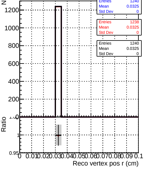
Recons Legend: DQM_original_step2_pt0p1to1_eta1p4to1p6 (blue line) DQM_mkFit_step2_pt0p1to1_eta1p4to1p6 (red line) DQM_pixelCPETemplate_step2_pt0p1to1_eta1p4to1p6 (black line)
