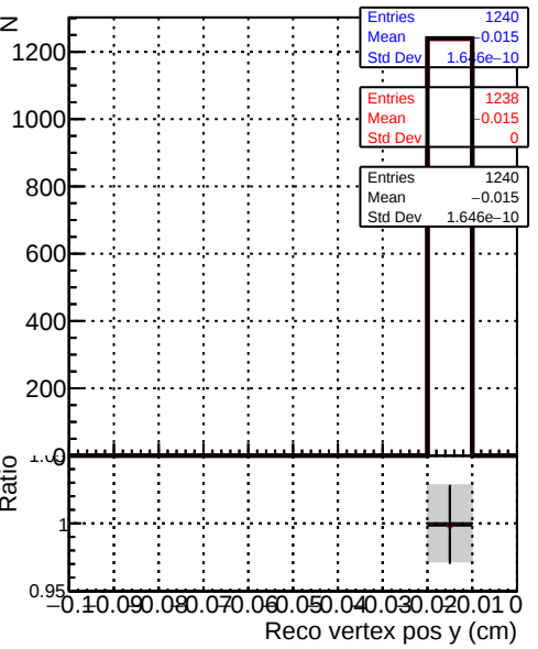
Recons Legend: DQM_original_step2_pt0p1to1_eta1p4to1p6 (blue line) DQM_mkFit_step2_pt0p1to1_eta1p4to1p6 (red line) DQM_pixelCPETemplate_step2_pt0p1to1_eta1p4to1p6 (black line)
