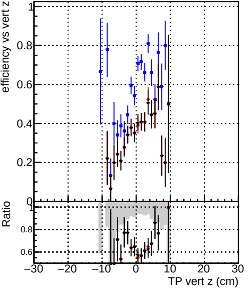
Efficiency vs. TP vert z (cm) Legend: DQM_original_step2_pt0p1to1_eta1p4to1p6 (blue circles) DQM_mkFit_step2_pt0p1to1_eta1p4to1p6 (red circles) DQM_pixelCPETemplate_step2_pt0p1to1_eta1p4to1p6 (black circles)
