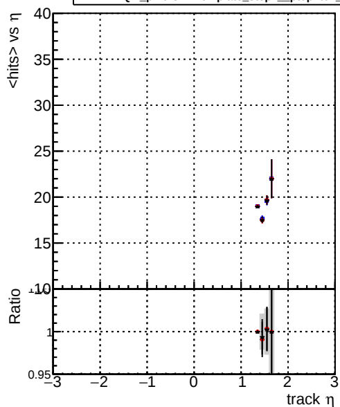
DQM_original_step2_pt0p1to1_eta1p4to1p6 DQM_mkFit_step2_pt0p1to1_eta1p4to1p6 DQM_pixelCPEtemplate_step2_pt0p1to1_eta1p4to1p6
