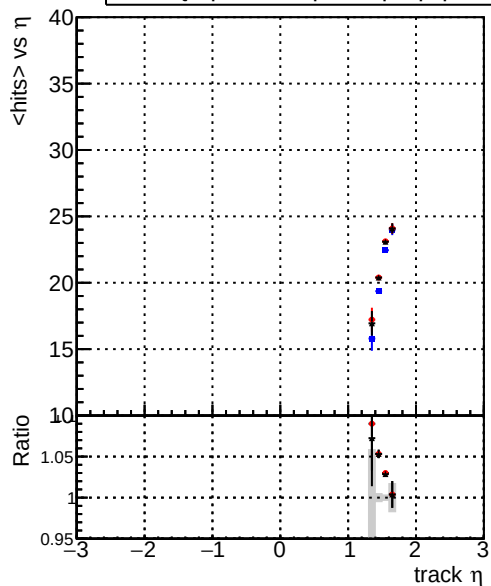
mean hits — DQM_original_step2_pt0p1to1_eta1p4to1p6 — DQM_mkFit_step2_pt0p1to1_eta1p4to1p6 — DQM_pixelCPETemplate_step2_pt0p1to1_eta1p4to1p6
