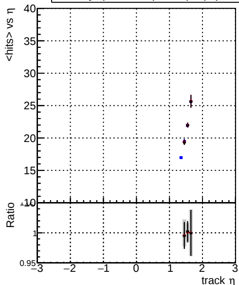
mean hits vs \eta — DQM_original_step2_pt0p1to1_eta1p4to1p6 — DQM_mkFit_step2_pt0p1to1_eta1p4to1p6 — DQM_pixelCPEtemplate_step2_pt0p1to1_eta1p4to1p6
