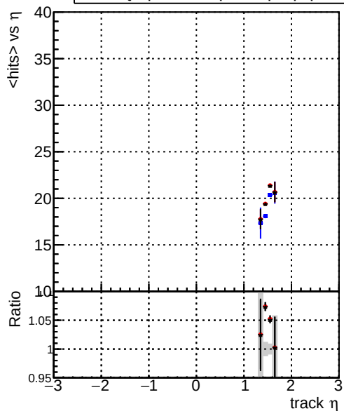
mean hit — DQM_original_step2_pt0p1to1_eta1p4to1p6 — DQM_mkFit_step2_pt0p1to1_eta1p4to1p6 — DQM_pixelCPETemplate_step2_pt0p1to1_eta1p4to1p6
