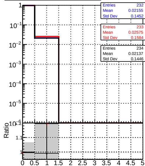
mean hits — DQM_original_step2_pt0p1to1_eta1p4to1p6 — DQM_mkFit_step2_pt0p1to1_eta1p4to1p6 — DQM_pixelCPETemplate_step2_pt0p1to1_eta1p4to1p6
