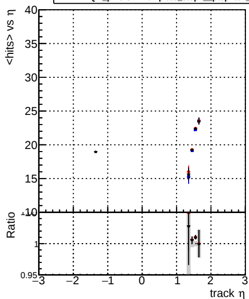
mean hits vs \eta — DQM_original_step2_pt0p1to1_eta1p4to1p6 — DQM_mkFit_step2_pt0p1to1_eta1p4to1p6 — DQM_pixelCPETemplate_step2_pt0p1to1_eta1p4to1p6
