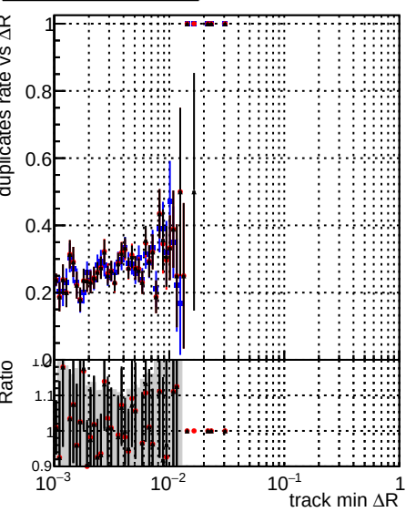
Legend: - DQM_original_step2_pt0p1to1_eta0p4to1p0 - DQM_mkFit_step2_pt0p1to1_eta0p4to1p0 - DQM_pixelCPETemplate_step2_pt0p1to1_eta0p4to1p0
