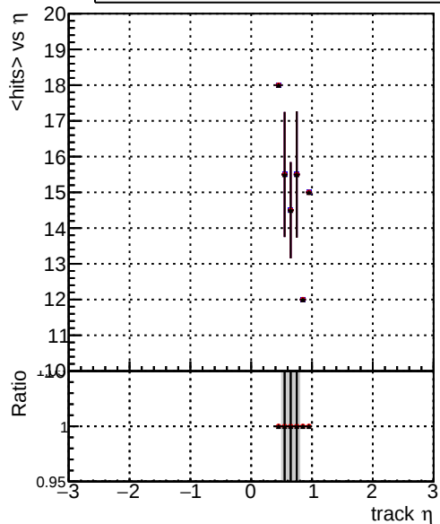
mean hits vs \eta DQM_original_step2_pt0p1to1_eta0p4to1p0 DQM_mkFit_step2_pt0p1to1_eta0p4to1p0 DQM_pixelCPEtemplate_step2_pt0p1to1_eta0p4to1p0
