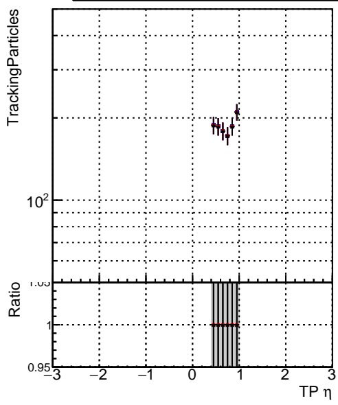
N of simulated tracks vs \eta Legend: DQM_original_step2_pt0p1to1_eta0p4to1p0 DQM_mkFit_step2_pt0p1to1_eta0p4to1p0 DQM_pixelCPEtemplate_step2_pt0p1to1_eta0p4to1p0
