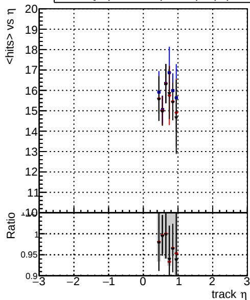
mean hit — DQM_original_step2_pt0p1to1_eta0p4to1p0 — DQM_mkFit_step2_pt0p1to1_eta0p4to1p0 — DQM_pixelCPEtemplate_step2_pt0p1to1_eta0p4to1p0
