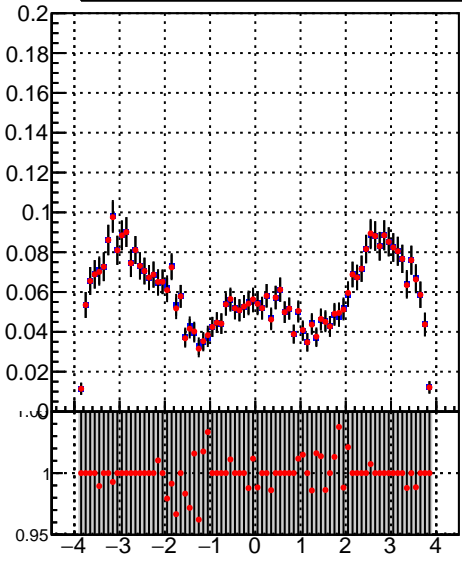
tracking_iters01LST_DNN_1000events tracking_iters01LST_preDNN_1000events
