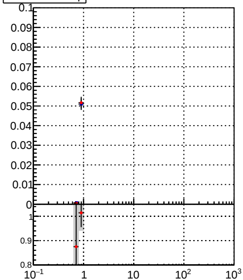
tracking_iters01LST_DNN_1000events tracking_iters01LST_preDNN_1000events
