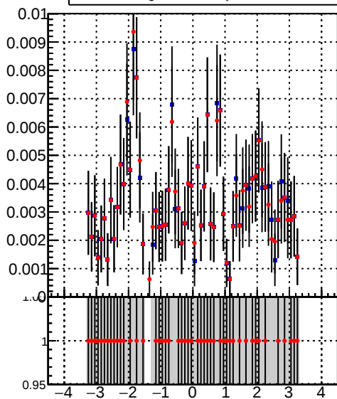
tracking_iters01LST_DNN_1000events tracking_iters01LST_preDNN_1000events
