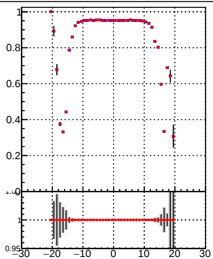
—●— tracking_iters01LST_DNN_1000events —●— tracking_iters01LST_preDNN_1000events
