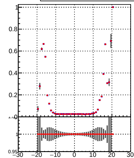
—●— tracking_iters01LST_DNN_1000events —●— tracking_iters01LST_preDNN_1000events
