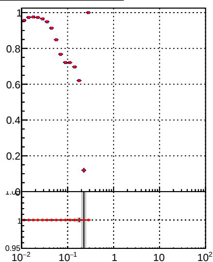
—●— tracking_iters01LST_DNN_1000events —●— tracking_iters01LST_preDNN_1000events
