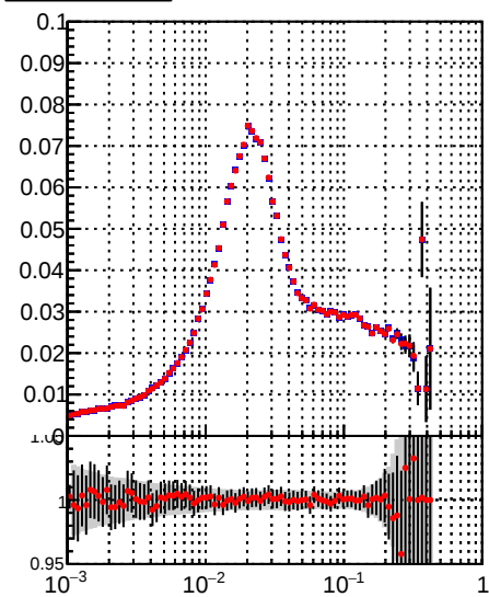
Fake rate vs \sqrt{s} tracking_iters01LST_DNN_1000events tracking_iters01LST_preDNN_1000events
