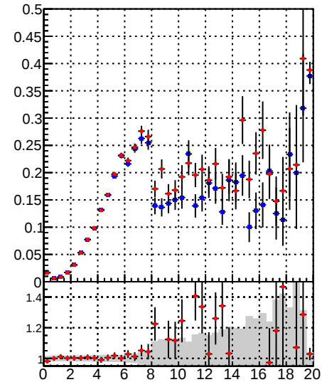
Fake rate vs. — tracking_iters01LST_DNN_1000events — tracking_iters01LST_preDNN_1000events
