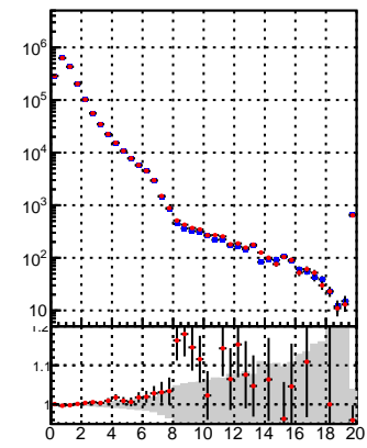
N of reco track vs. \chi^2 for tracking_iters01LST_DNN_1000events and tracking_iters01LST_preDNN_1000events
