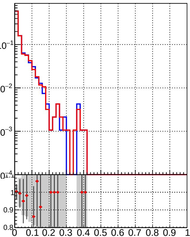
RecoPVAssoc2GenPVMatched_Missing
