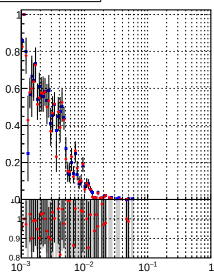
■ tracking_iters01LST_DNN_1000events ● tracking_iters01LST_predDNN_1000events
