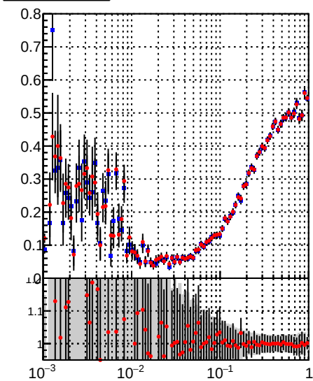
■ tracking_iters01LST_DNN_1000events ● tracking_iters01LST_predDNN_1000events
