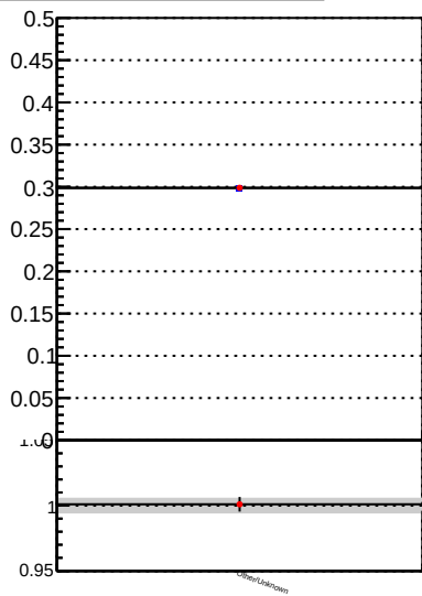
Fake rate vs. — tracking_iters01LST_DNN_1000events — tracking_iters01LST_preDNN_1000events
