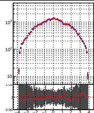
tracking_Iters01LST_DNN_1000events tracking_Iters01LST_preDNN_1000events
