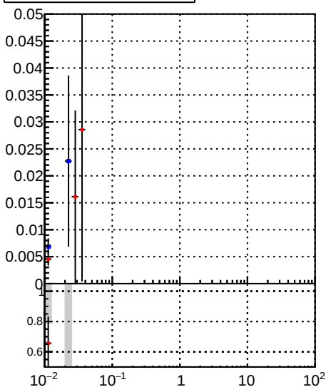
■ tracking_iters01LST_DNN_1000events ● tracking_iters01LST_preDNN_1000events
