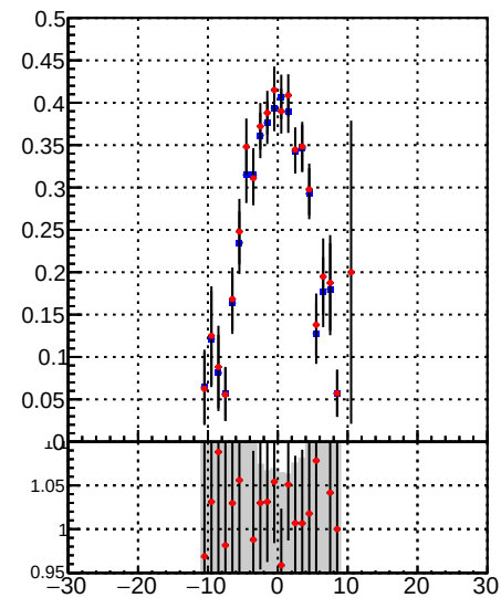
tracking_Iters01LST_DNN_1000events tracking_Iters01LST_preDNN_1000events
