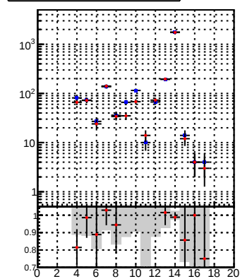
tracking_Iters01LST_DNN_1000events tracking_Iters01LST_preDNN_1000events
