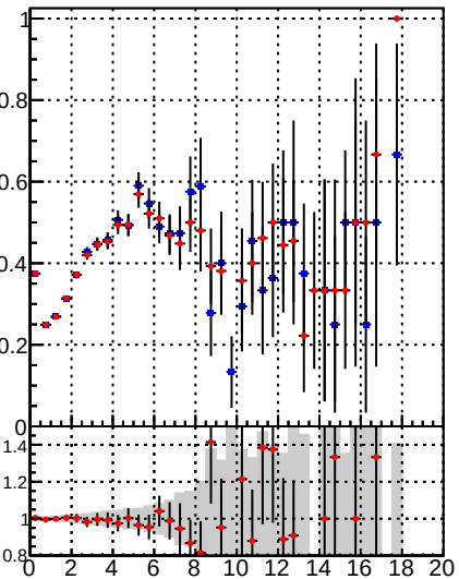
Fake rate vs. — tracking_iters01LST_DNN_1000events — tracking_iters01LST_preDNN_1000events
