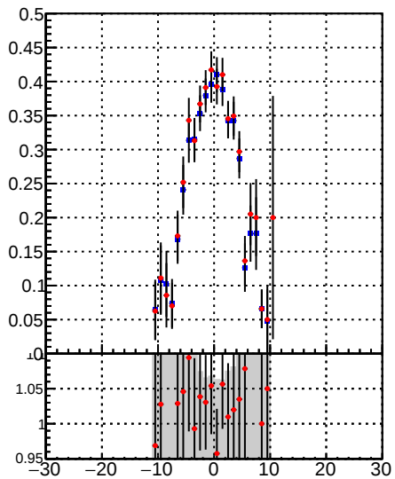
tracking_Iters01LST_DNN_1000events tracking_Iters01LST_preDNN_1000events
