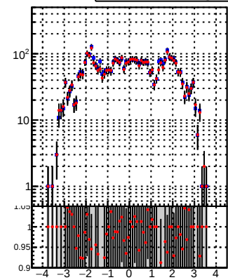
tracking_Iters01LST_DNN_1000events tracking_Iters01LST_preDNN_1000events
