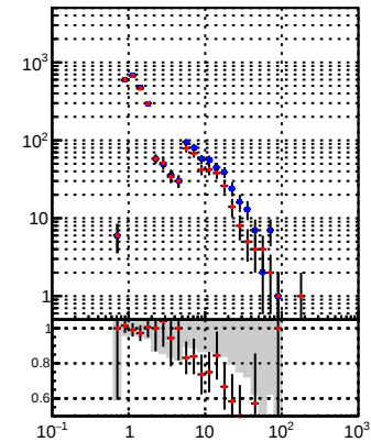
tracking_Iters01LST_DNN_1000events tracking_Iters01LST_preDNN_1000events
