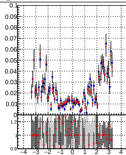
■ tracking_iters01LST_DNN_1000events ■ tracking_iters01LST_preDNN_1000events
