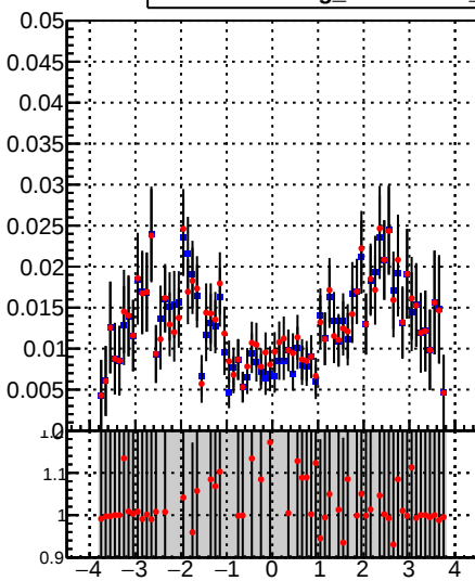
■ tracking_iters01LST_DNN_1000events ■ tracking_iters01LST_preDNN_1000events
