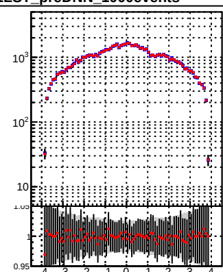
tracking_Iters01LST_DNN_1000events tracking_Iters01LST_preDNN_1000events
