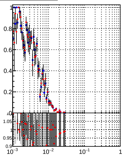
■ tracking_iters01LST_DNN_1000events ■ tracking_iters01LST_preDNN_1000events
