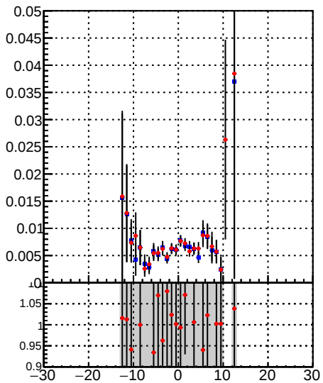
tracking_Iters01LST_DNN_1000events tracking_Iters01LST_preDNN_1000events
